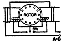
Shaded-pole induction-motor circuit (reversible).
